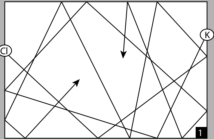
brownian movement
