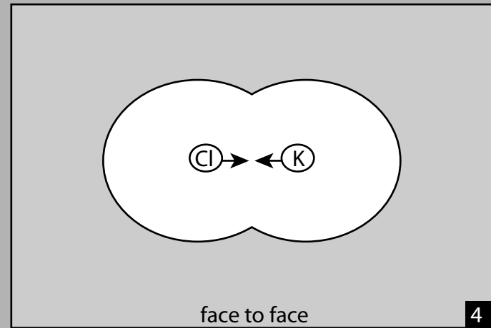
brownian movement
